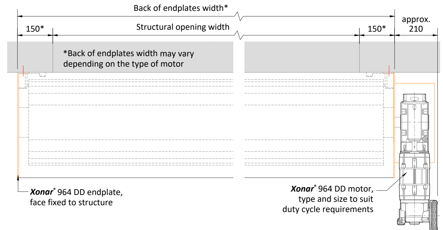
Plan Through: B-B (scale 1:10)
