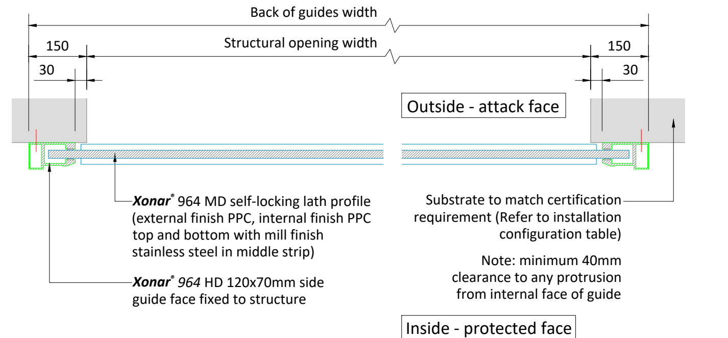
Plan Through: B-B (scale 1:10)
