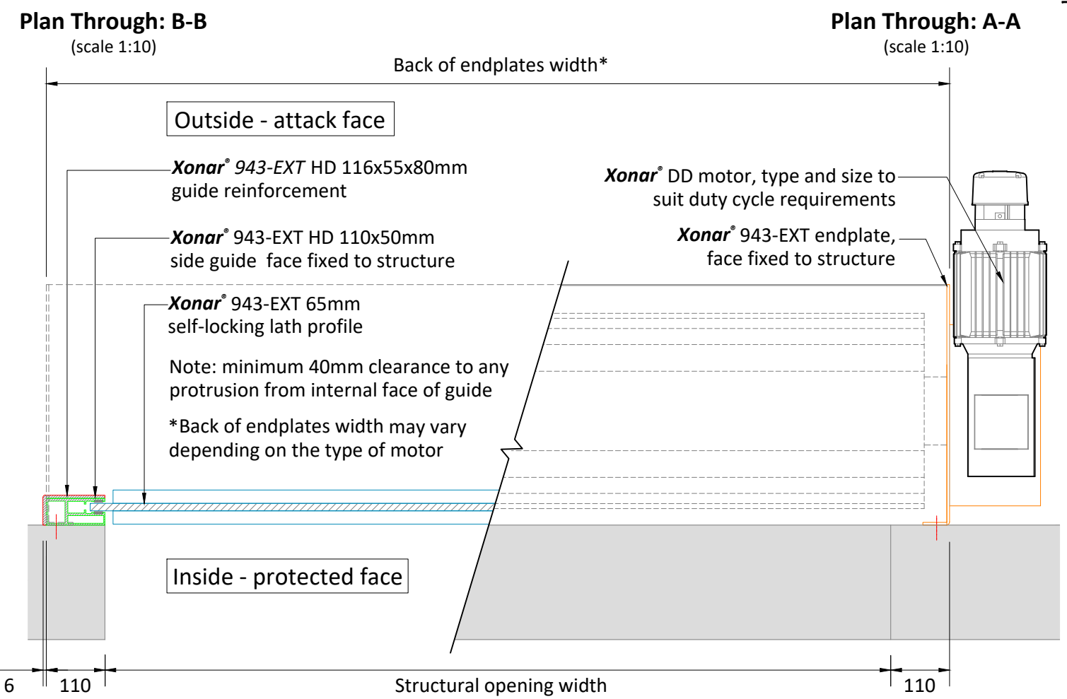
Xonar® 943-EXT-DD guide: (scale 1:5)
