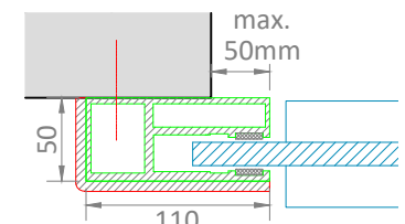
Xonar® 943 110x50 HD guide (BS EN 12424, Wind load performance up to Class 5)
