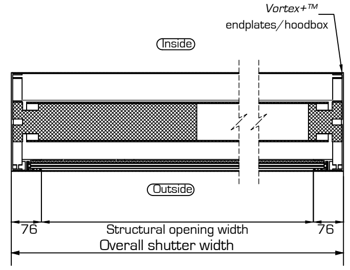
Plan through: A-A (scale - 1:10)
