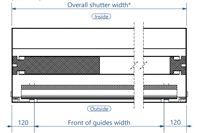
Plan through: A-A (scale - 1:10)
