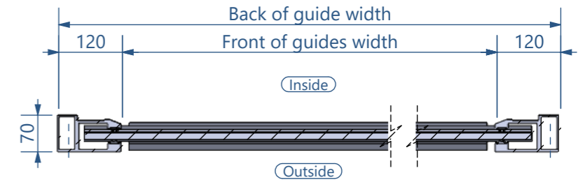
Plan through: B-B (scale - 1:10)
