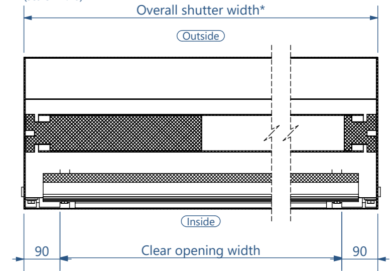
Plan through: A-A (scale - 1:10)
