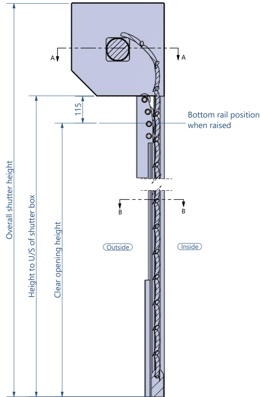
Section (scale - 1:10)
