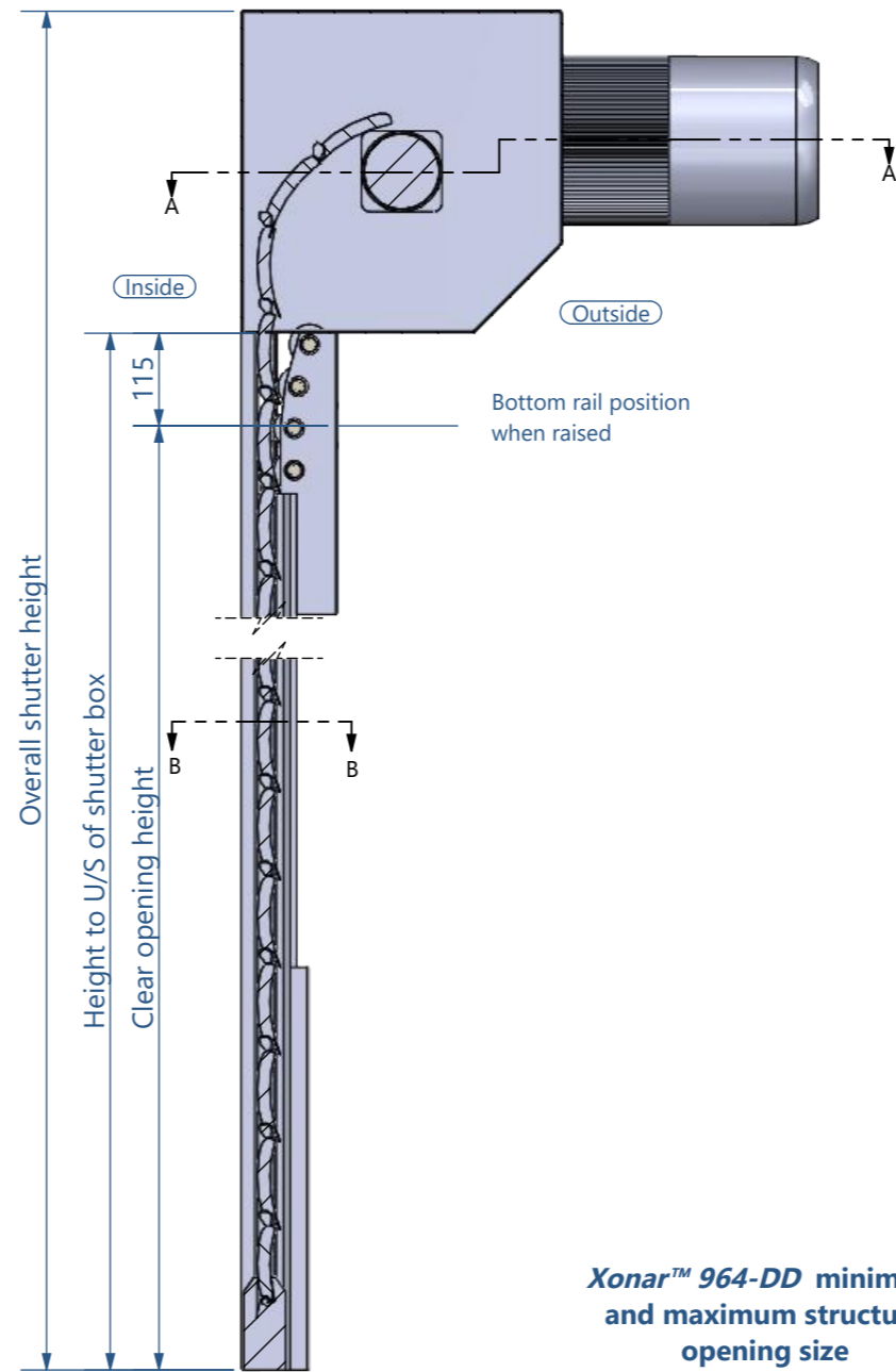
Section (scale - 1:10)
