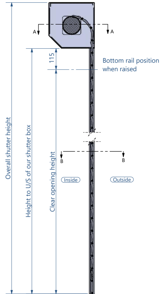
Section (scale - 1:10)
