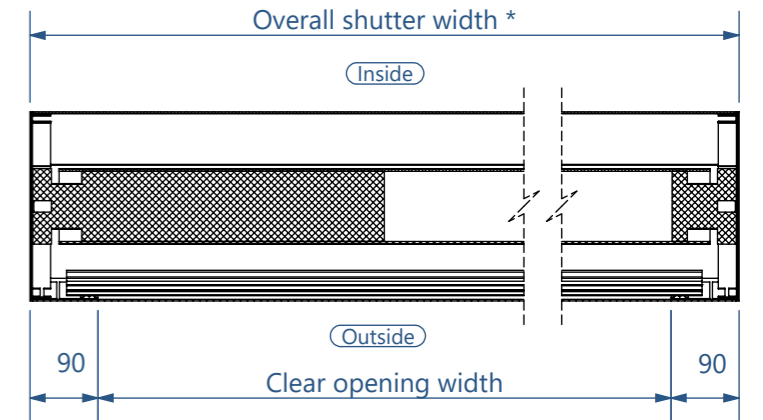
Plan through: A-A (scale - 1:10)
