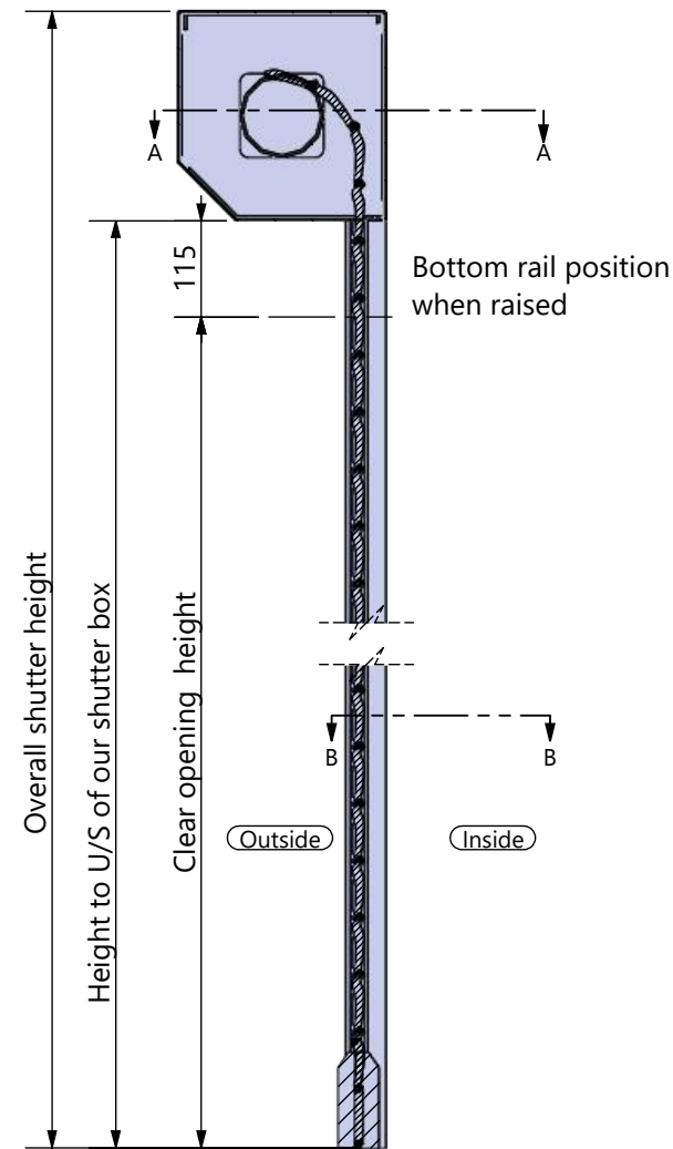
Section (scale - 1:10)
