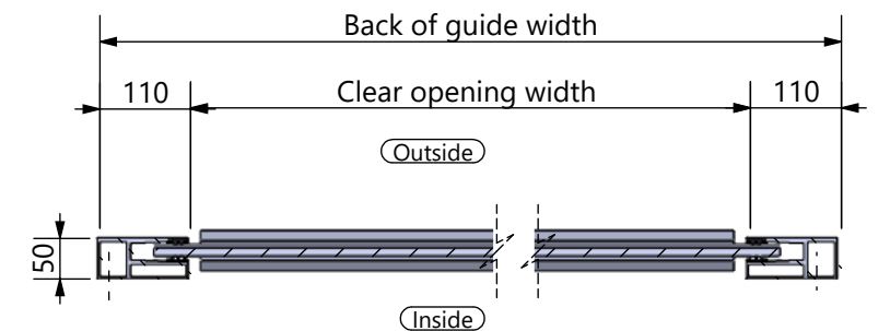
Plan through: B-B (scale - 1:10)
