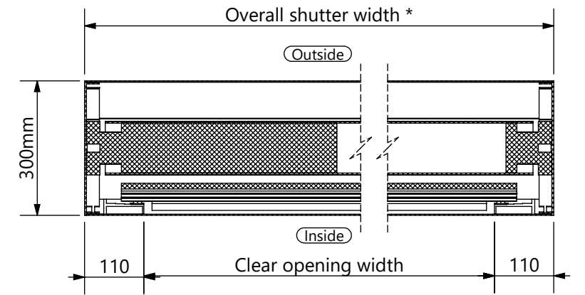
Plan through: A-A (scale - 1:10)
