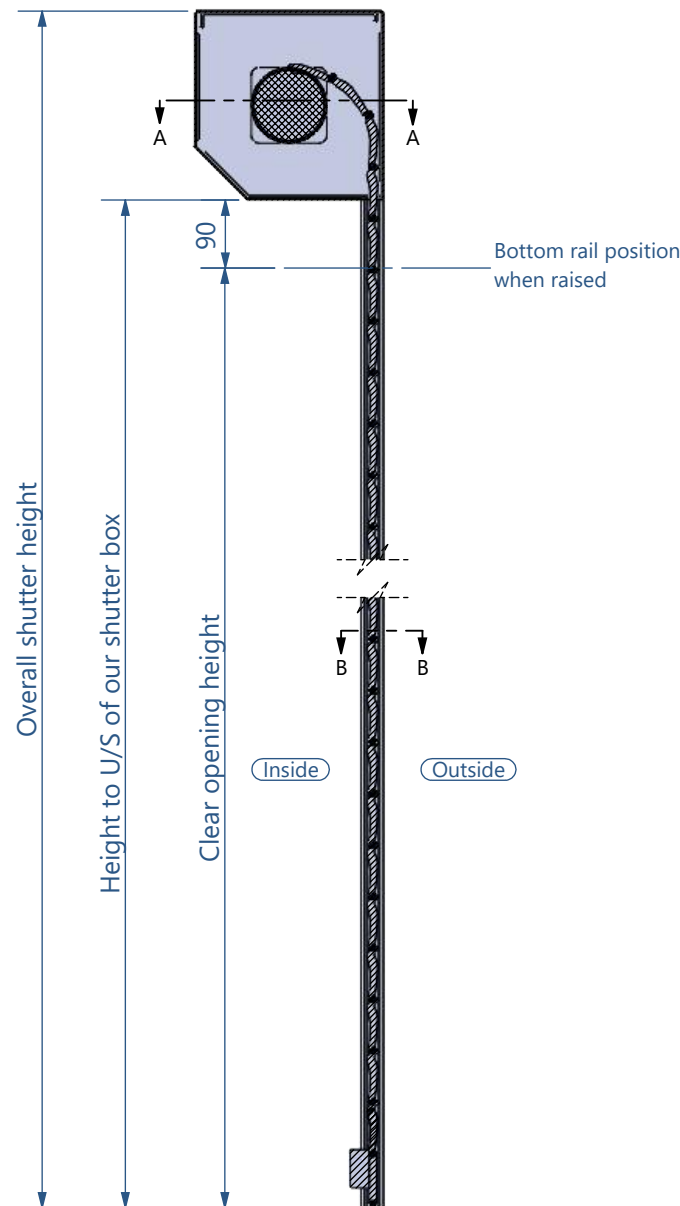
Section (scale - 1:10)
